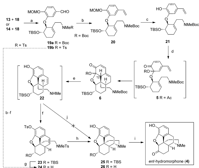
Scheme 3. a) TMAD, \text{PBu}_3 , 81–85%; b) \text{CH}_3\text{PPh}_2 , n\text{BuLi} , THF, -78^\circ\text{C} to 0^\circ\text{C} then reflux for 4 h, 82–88%; c) \text{ZnBr}_2 , \text{CH}_3(\text{CH}_2)_{10}\text{CH}_2\text{SH} , \text{CH}_2\text{Cl}_2 , RT, 10 min, 92%; d) \text{Pb}(\text{OAc})_4 , DCE, reflux, 4 h, 50%; e) TFA, \text{CH}_2\text{Cl}_2 , 0^\circ\text{C} , 15 min; f) \text{TsCl} , \text{Et}_3\text{N} , \text{CH}_2\text{Cl}_2 , 0^\circ\text{C} to RT, 45% over two steps; g) TBAF, THF, RT, 86%; h) \text{Li} , t\text{BuOH} , \text{NH}_3(\text{liq}) , THF, -78^\circ\text{C} , 10 min [82–86% for 23 to 25 ; 93% for 24 to 26 ]; i) t\text{BuOK} , \text{PhCOPh} , \text{PhCH}_3/\text{DME} , 85^\circ\text{C} , 8 h, 44%; j) 1. \text{Hg}(\text{OCOCF}_3)_2 , \text{CH}_3\text{CN} RT; 2. \text{NaBH}_4 , THF, -78^\circ\text{C} to RT. DCE = 1,2-dichloroethane, DME = dimethoxyethane, TBAF = tert - n -butylammonium fluoride, TMAD = N,N,N',N' -tetramethylazodicarboxamide.
