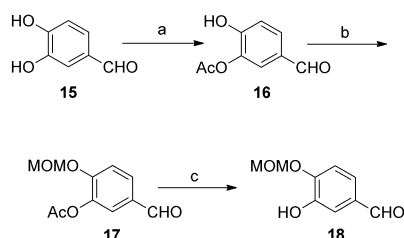
Scheme 2. a) Ac 2 O, NaOH, THF, 0°C, 82–85%; b) MOMCl, K 2 CO 3 , DMF, 0°C to RT, 76–80%; c) K 2 CO 3 , MeOH, RT, 88–90%. DMF = N,N -dimethylformamide.
