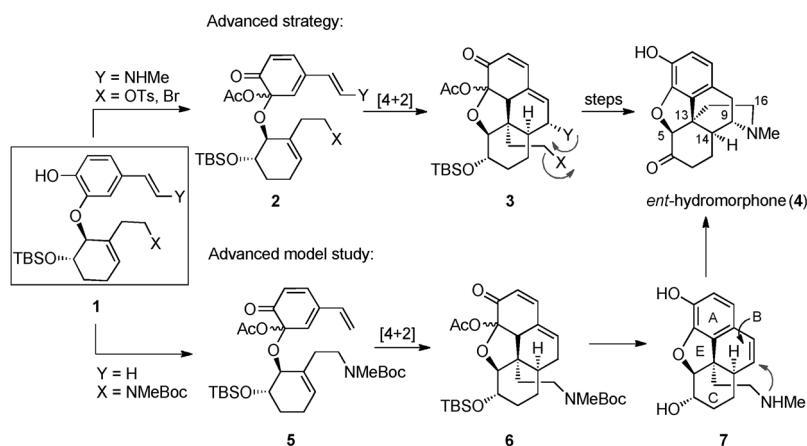
Figure 1. Advanced strategy to access morphinans by cycloaddition to construct ring B.
