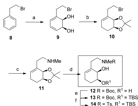
Scheme 1. a) E. coli JM 109 (pDTG601A), 10–15 g L -1 ; b) 1. potassium azodicarboxylate, AcOH, MeOH, 0°C, 83%; 2. 2,2-dimethoxypropane, acetone, p TsOH, 80%; c) MeNH 2 , K 2 CO 3 , THF, sealed tube, 93%; d) 1. 3 M HCl, EtOH; 2. Boc 2 O, NaHCO 3 , EtOH, 74% (2 steps); e) TBSCl, imidazole, CH 2 Cl 2 , -78°C to RT, 92%; f) 1. TFA, CH 2 Cl 2 , 0°C; 2. TsCl, Et 3 N, CH 2 Cl 2 , RT, 86% over two steps. Boc = tert -butoxycarbonyl, TBS = tert -butyldimethylsilyl, TFA = trifluoroacetic acid, Ts = 4-toluenesulfonyl.
